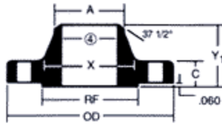
WELD NECK
